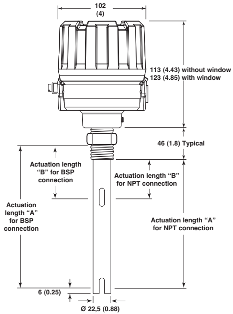
962 - Threaded connection
