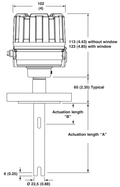
962 - Flanged connection
