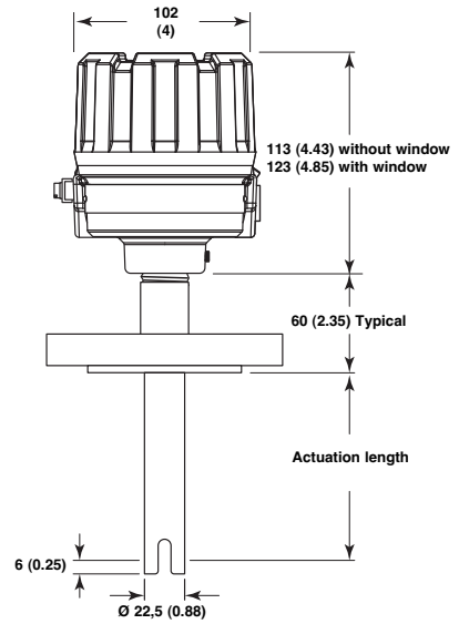
961 - Flanged connection
