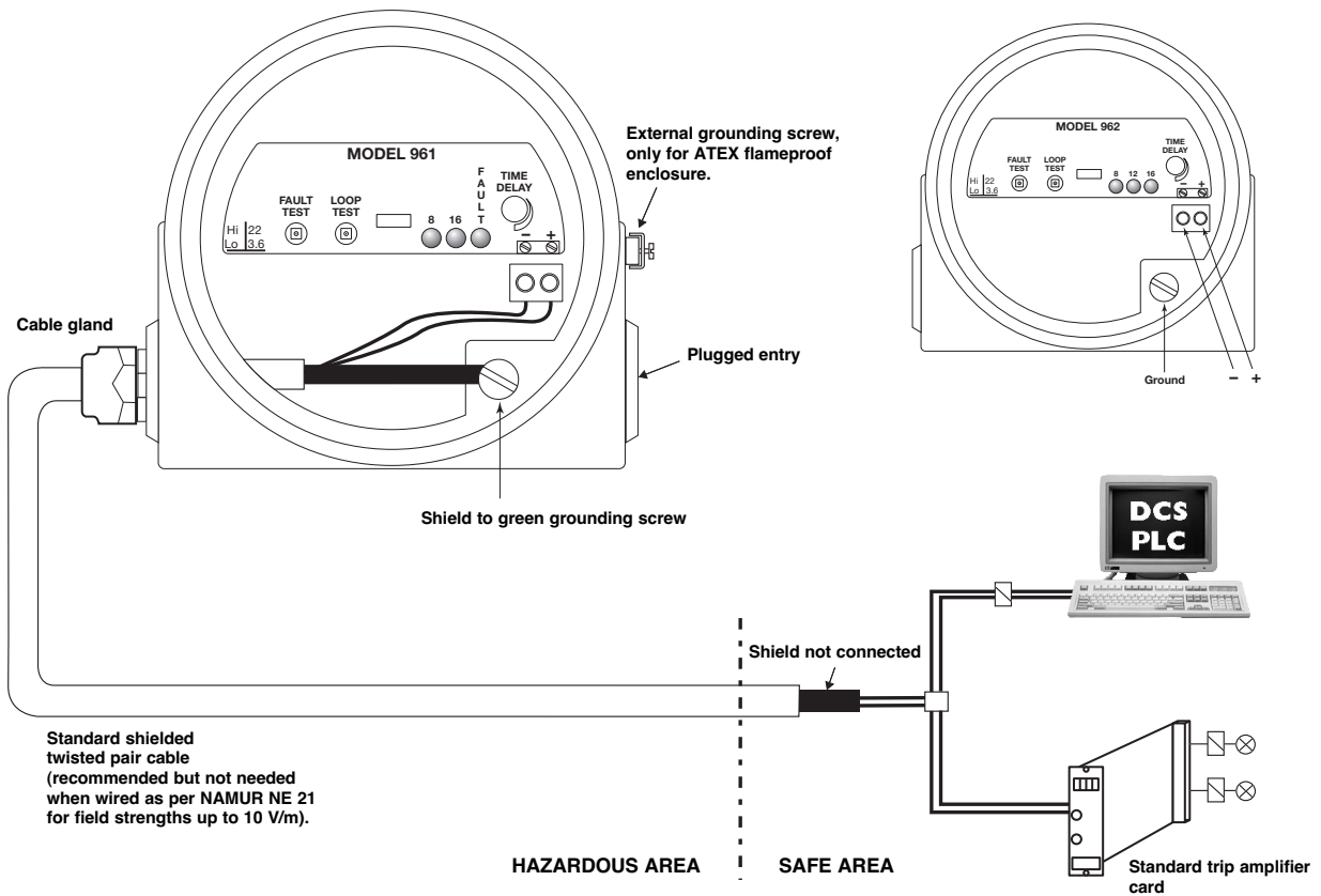
Echotel® 961 electronics
